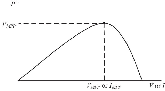
Fig. 2. Characteristic PV array power curve
