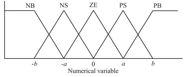
Fig. 5. Membership function for inputs and output of fuzzy logic controller
