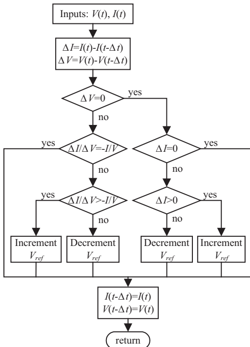
Fig. 4. IncCond algorithm as shown in [29, 32, 33, 36]
