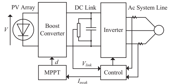
Fig. 7. Topology for dc link capacitor droop control as shown in [71]
