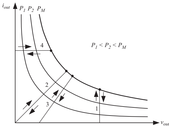
Fig. 8. Different load types: 1-voltage-source, 2-resistive, 3-resistive and voltage-source, 4-current-source, as shown in [78]
